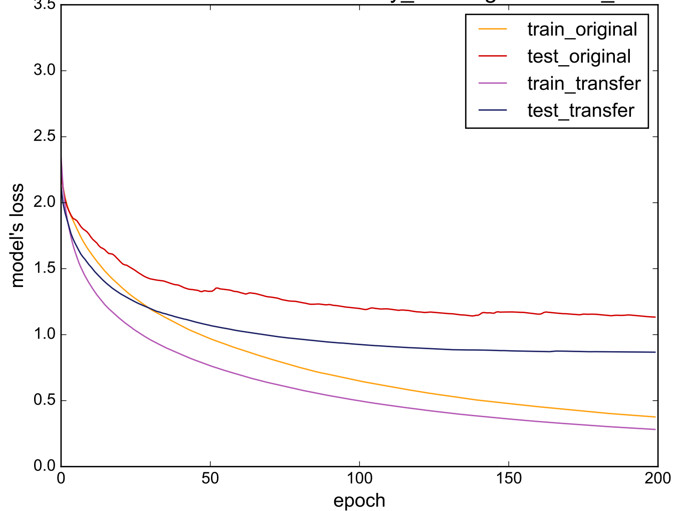
Source: uWaveGestureLibrary_Y - Target: Cricket_Y
