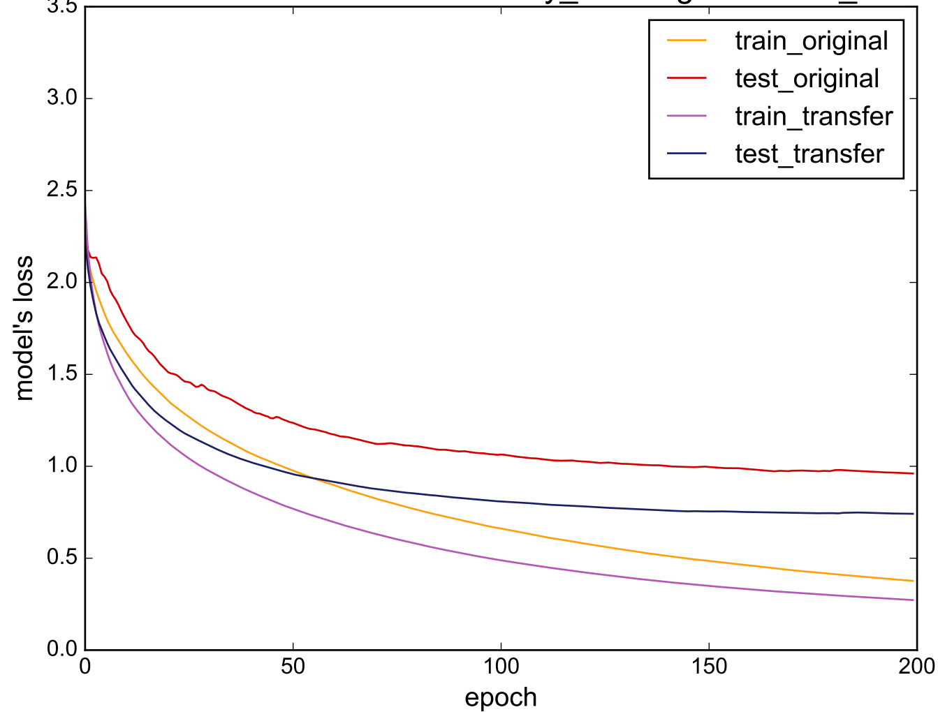
Source: uWaveGestureLibrary_Y - Target: Cricket_Z
