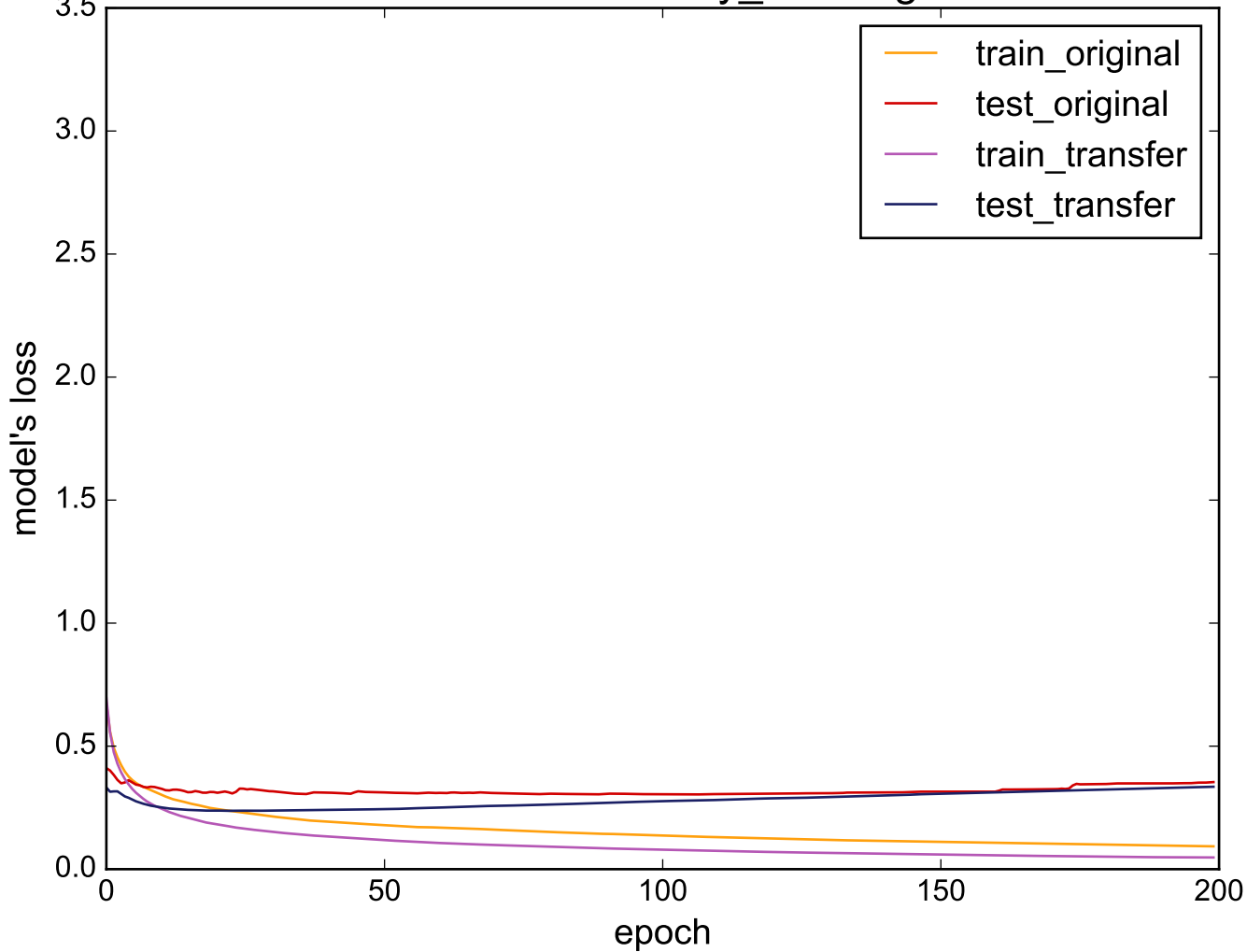
Source: uWaveGestureLibrary_Y - Target: ECG5000
