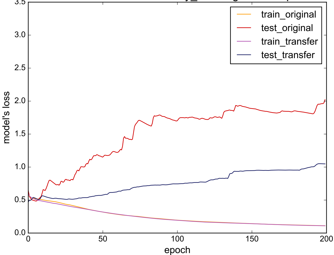
Source: uWaveGestureLibrary_Y - Target: Earthquakes
