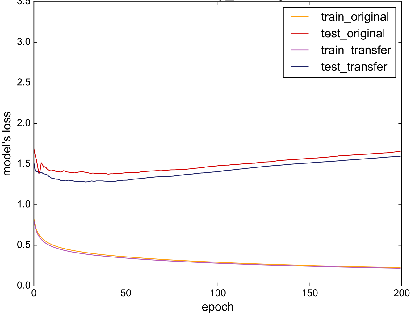
Source: uWaveGestureLibrary_Y - Target: ElectricDevices
