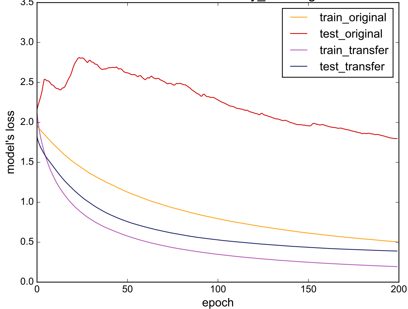
Source: uWaveGestureLibrary_Y - Target: FISH
