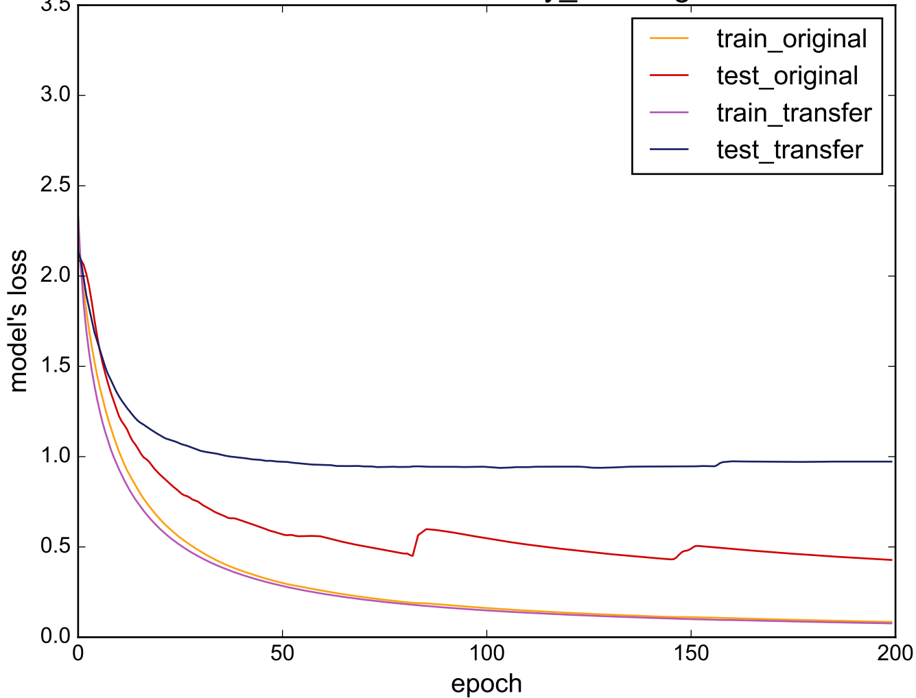
Source: uWaveGestureLibrary_Y - Target: FaceAll
