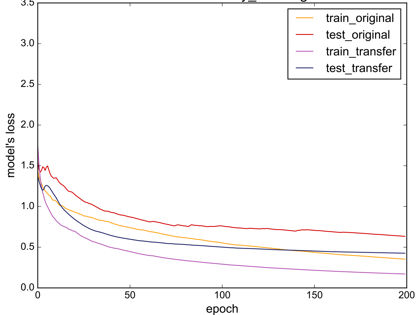
Source: uWaveGestureLibrary_Y - Target: FaceFour
