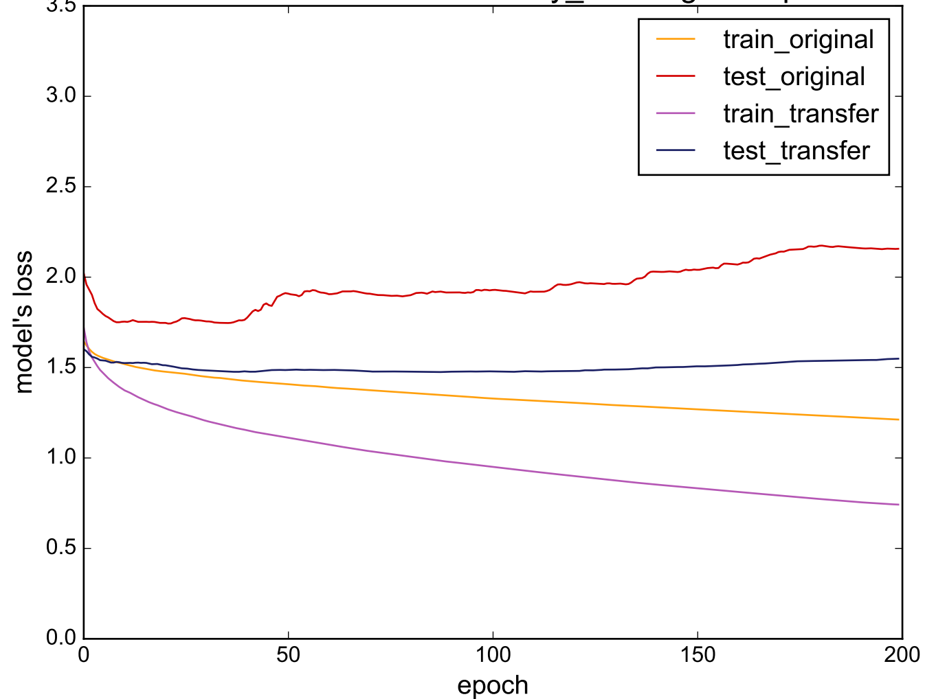
Source: uWaveGestureLibrary_Y - Target: Haptics
