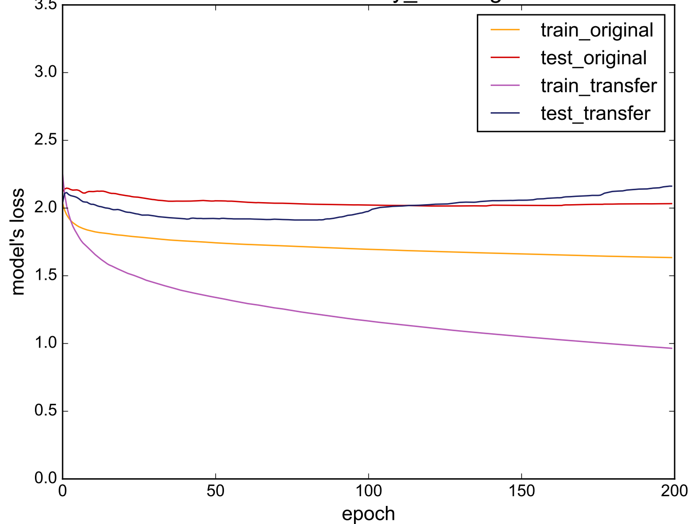
Source: uWaveGestureLibrary_Y - Target: InlineSkate
