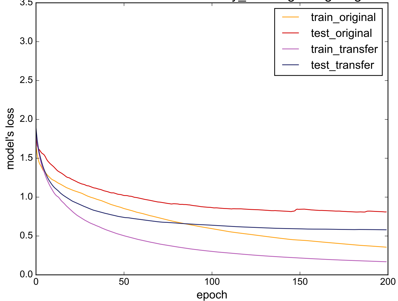
Source: uWaveGestureLibrary_Y - Target: Lighting7
