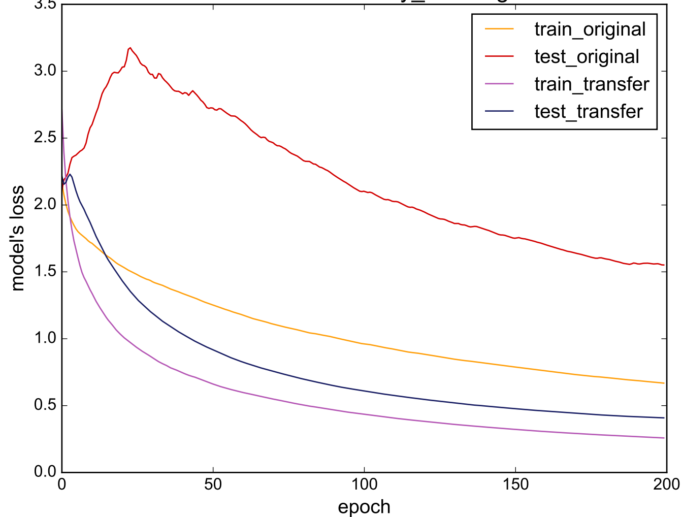
Source: uWaveGestureLibrary_Y - Target: MALLAT
