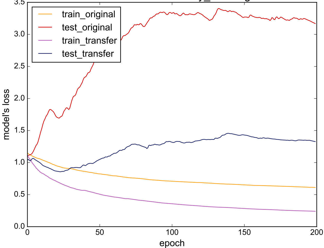
Source: uWaveGestureLibrary_Y - Target: Meat
