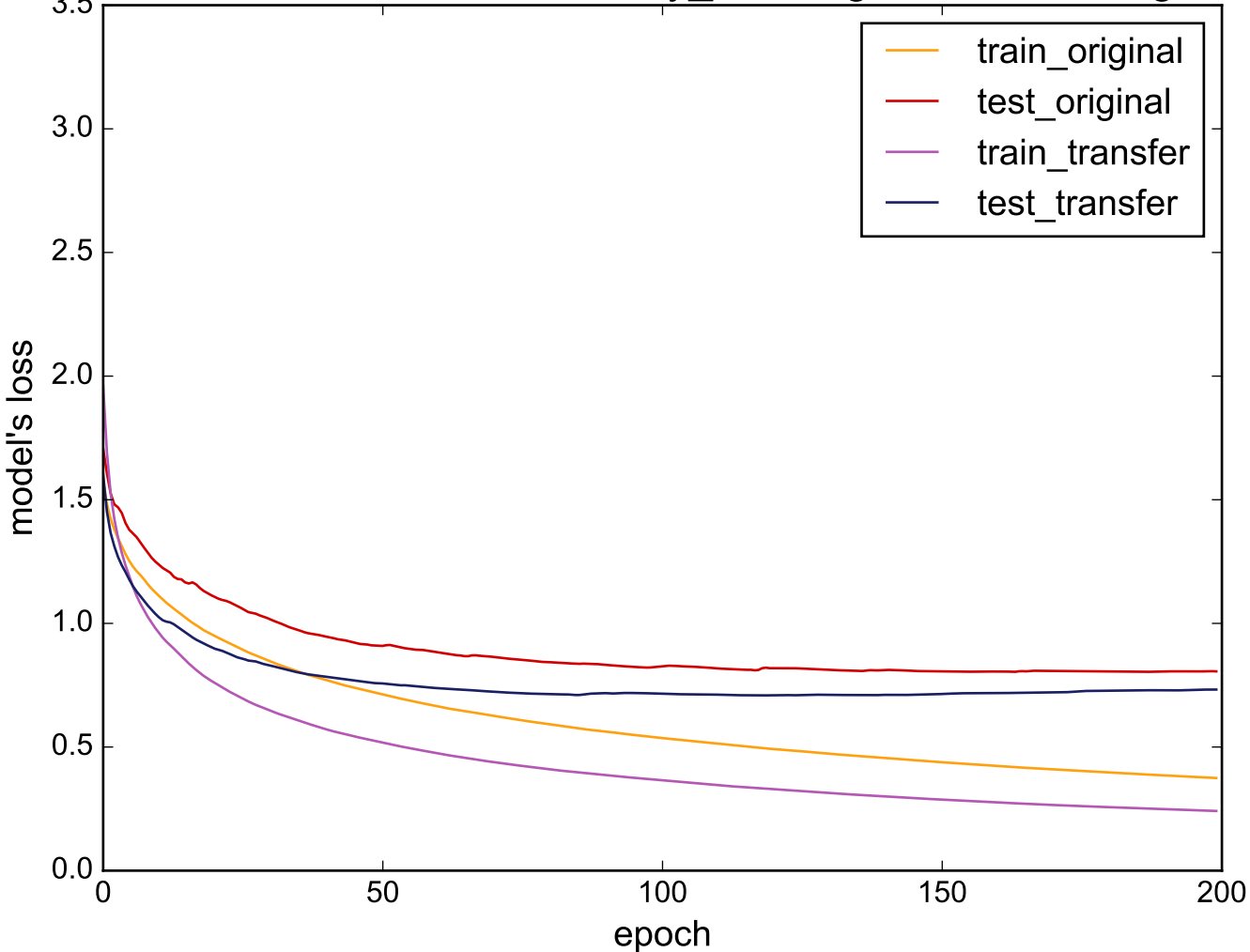
Source: uWaveGestureLibrary_Y - Target: MedicalImages
