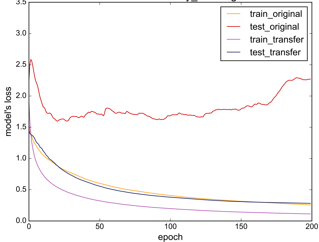
Source: uWaveGestureLibrary_Y - Target: OSULeaf
