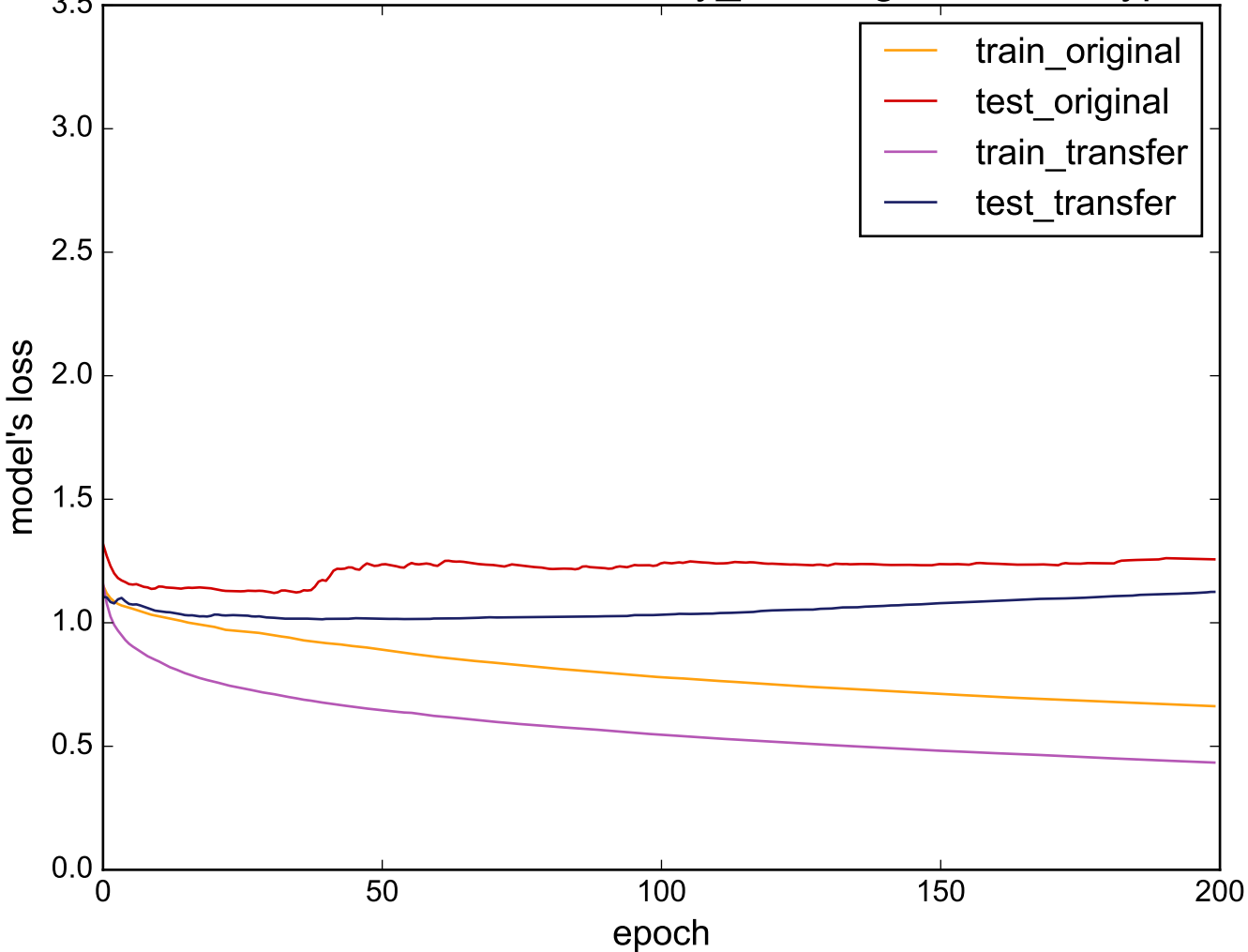
Source: uWaveGestureLibrary_Y - Target: ScreenType
