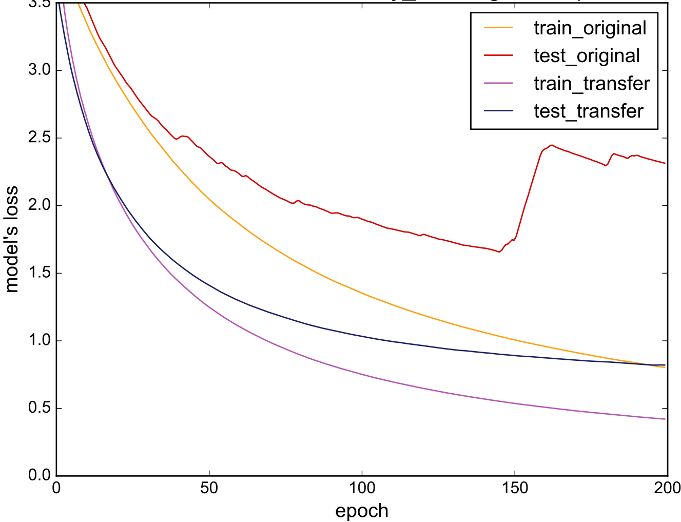
Source: uWaveGestureLibrary_Y - Target: ShapesAll
