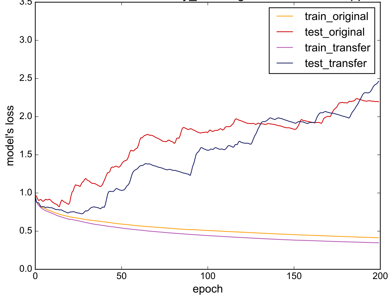
Source: uWaveGestureLibrary_Y - Target: SmallKitchenAppliances
