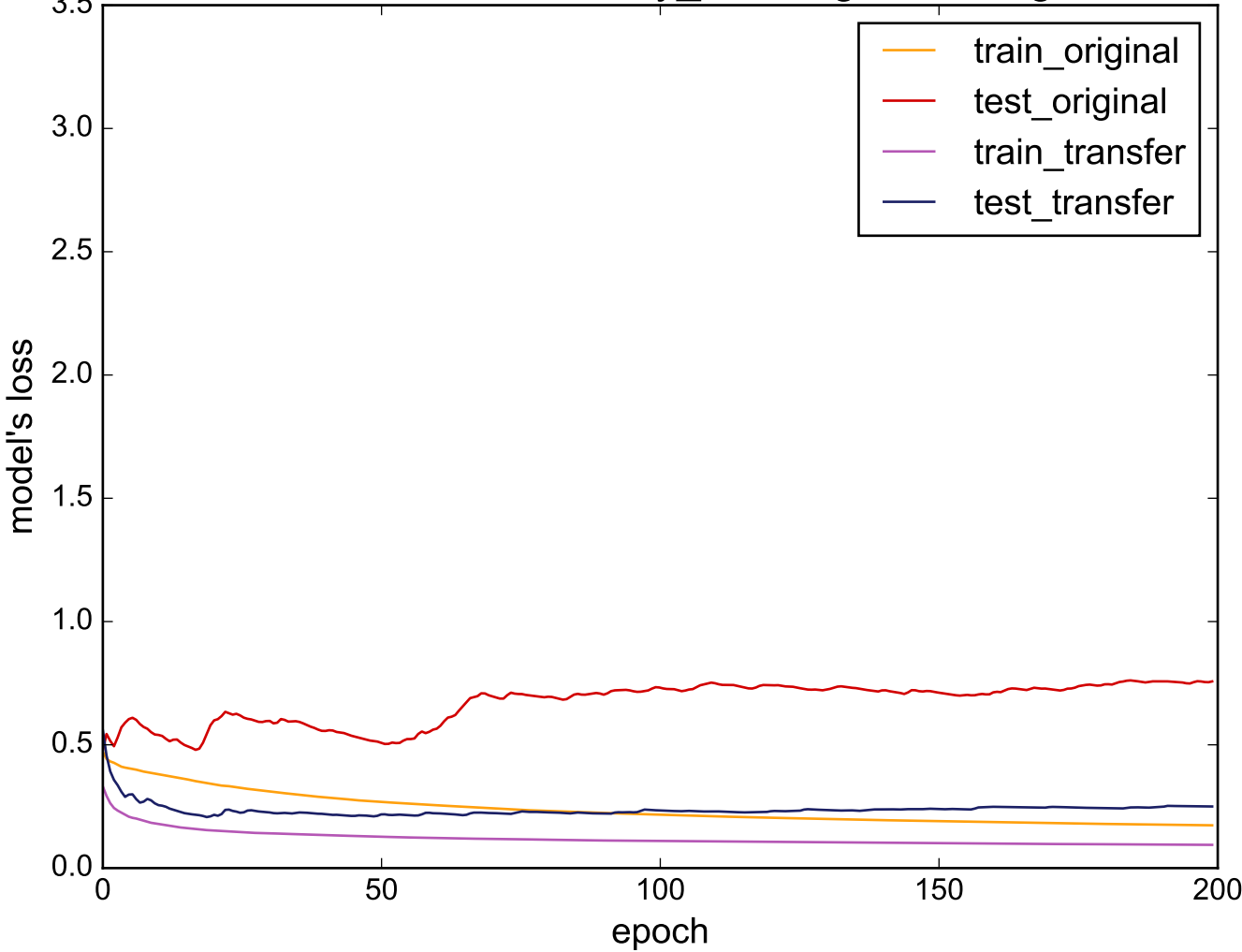
Source: uWaveGestureLibrary_Y - Target: StarLightCurves
