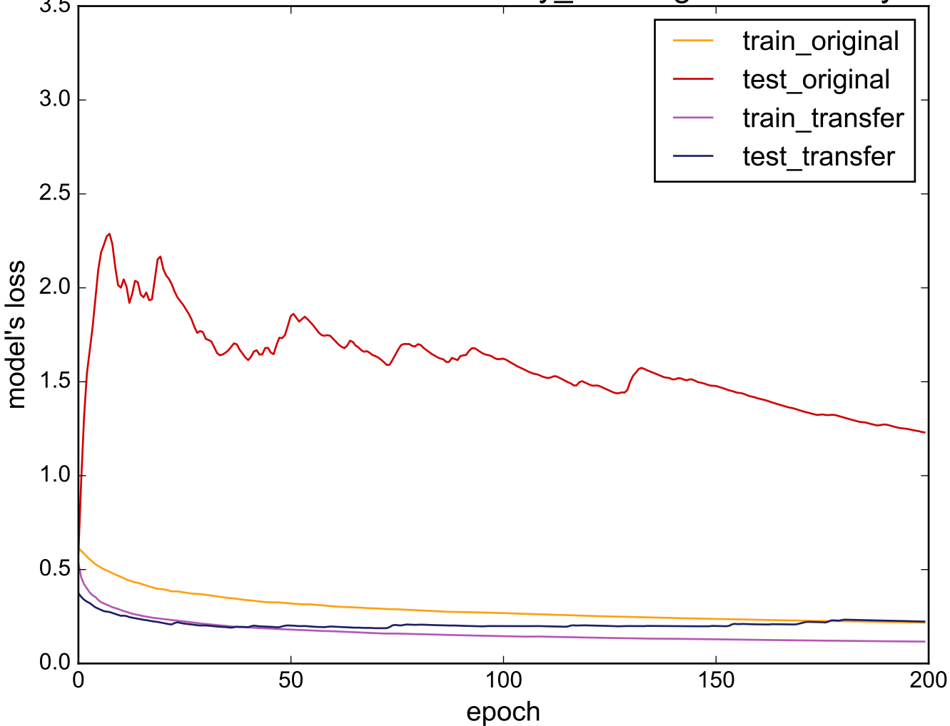
Source: uWaveGestureLibrary_Y - Target: Strawberry
