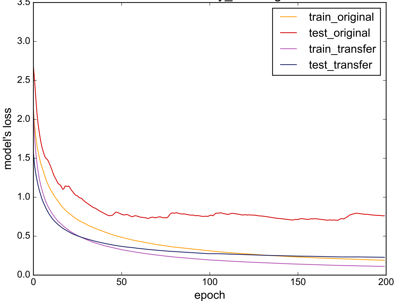
Source: uWaveGestureLibrary_Y - Target: SwedishLeaf
