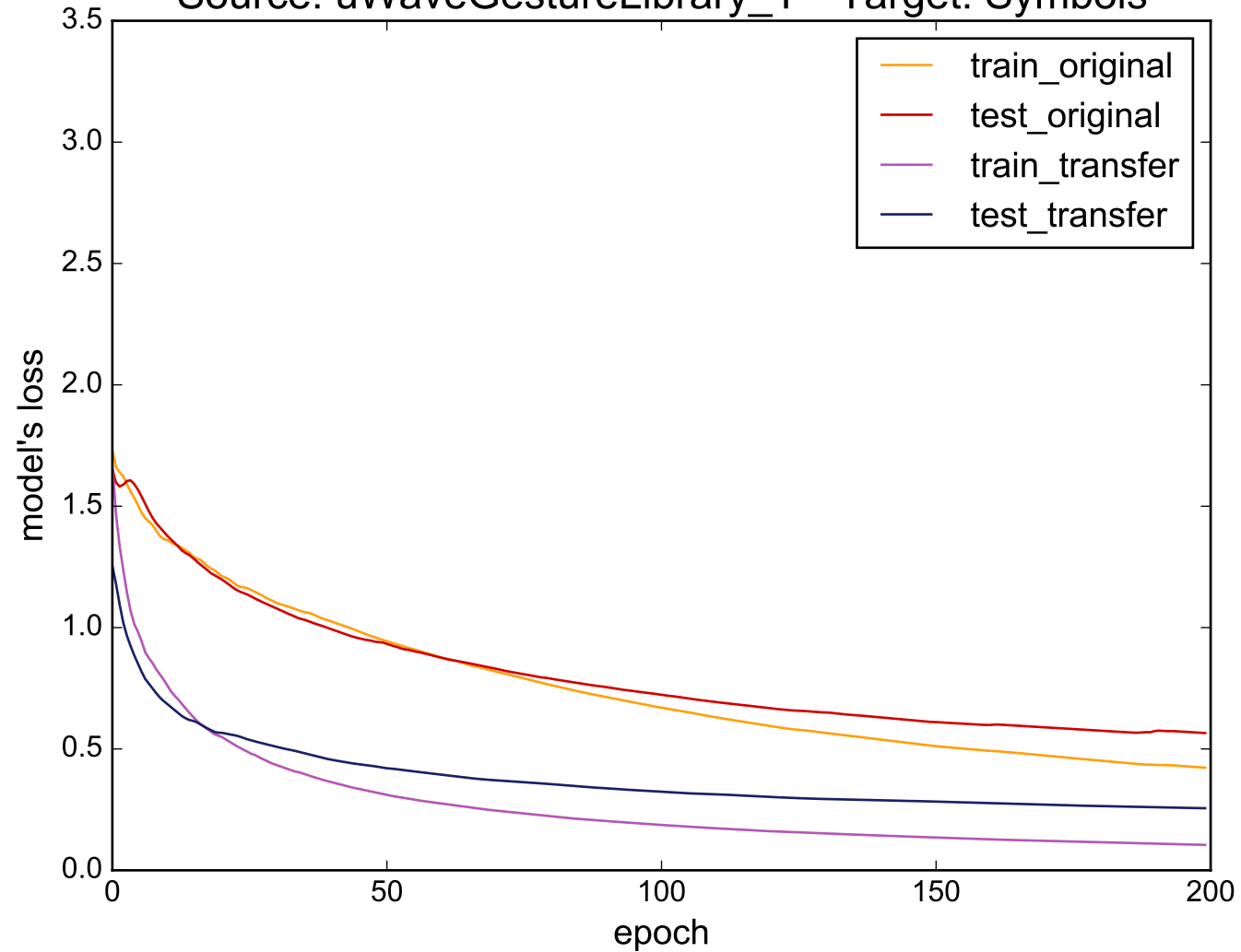
Source: uWaveGestureLibrary_Y - Target: Symbols
