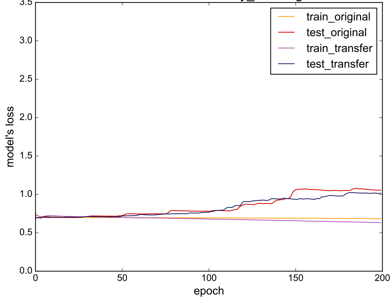
Source: uWaveGestureLibrary_Y - Target: Wine
