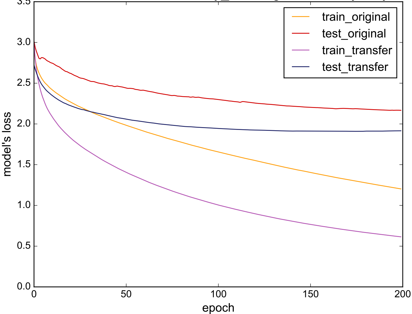
Source: uWaveGestureLibrary_Y - Target: WordsSynonyms
