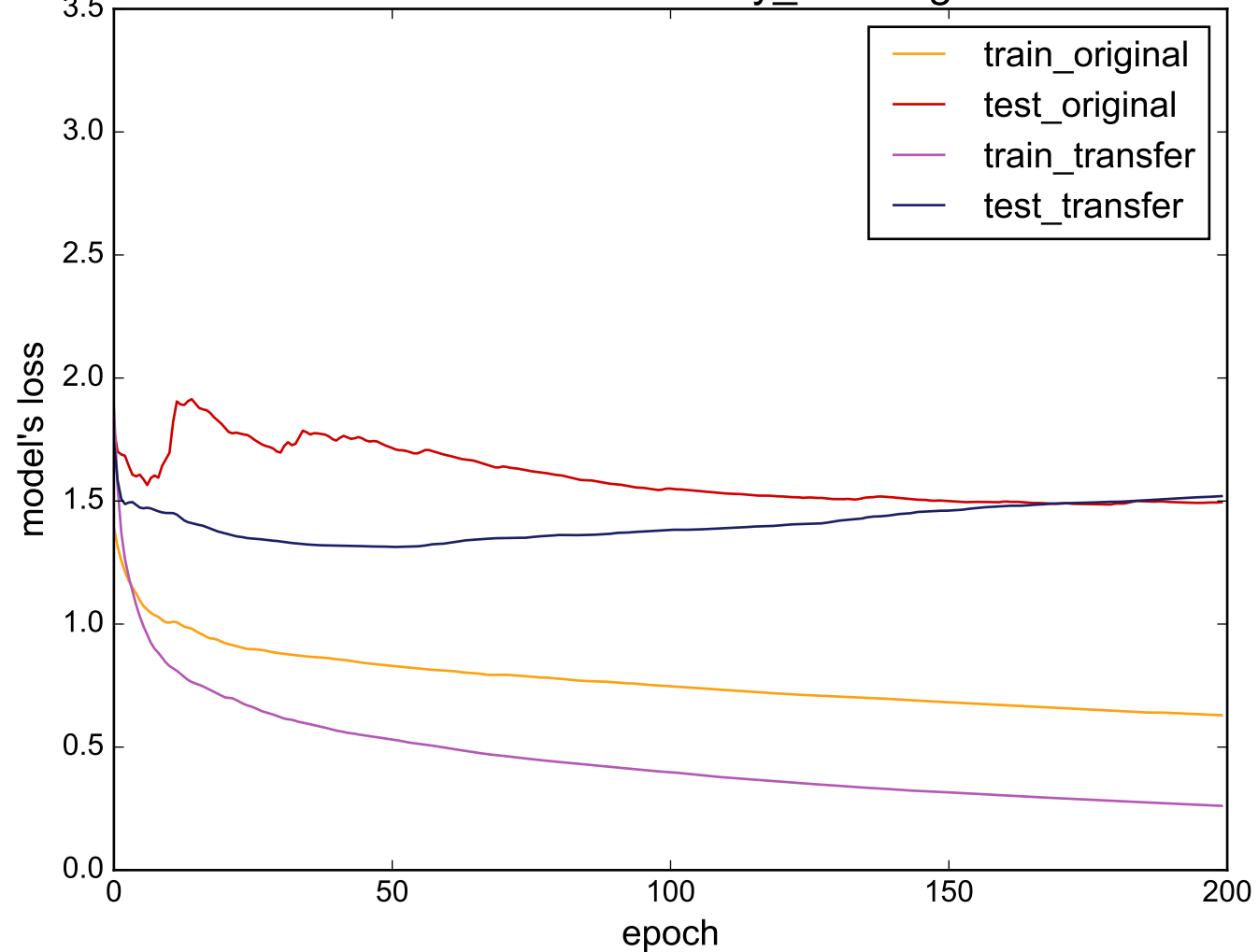
Source: uWaveGestureLibrary_Y - Target: Worms
