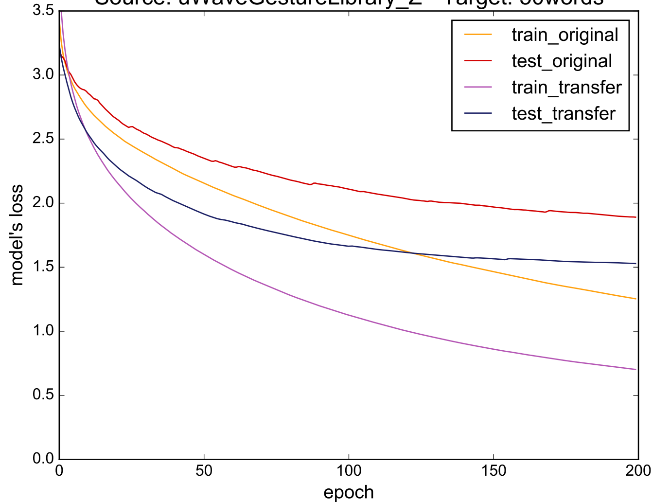
Source: uWaveGestureLibrary_Z - Target: 50words
