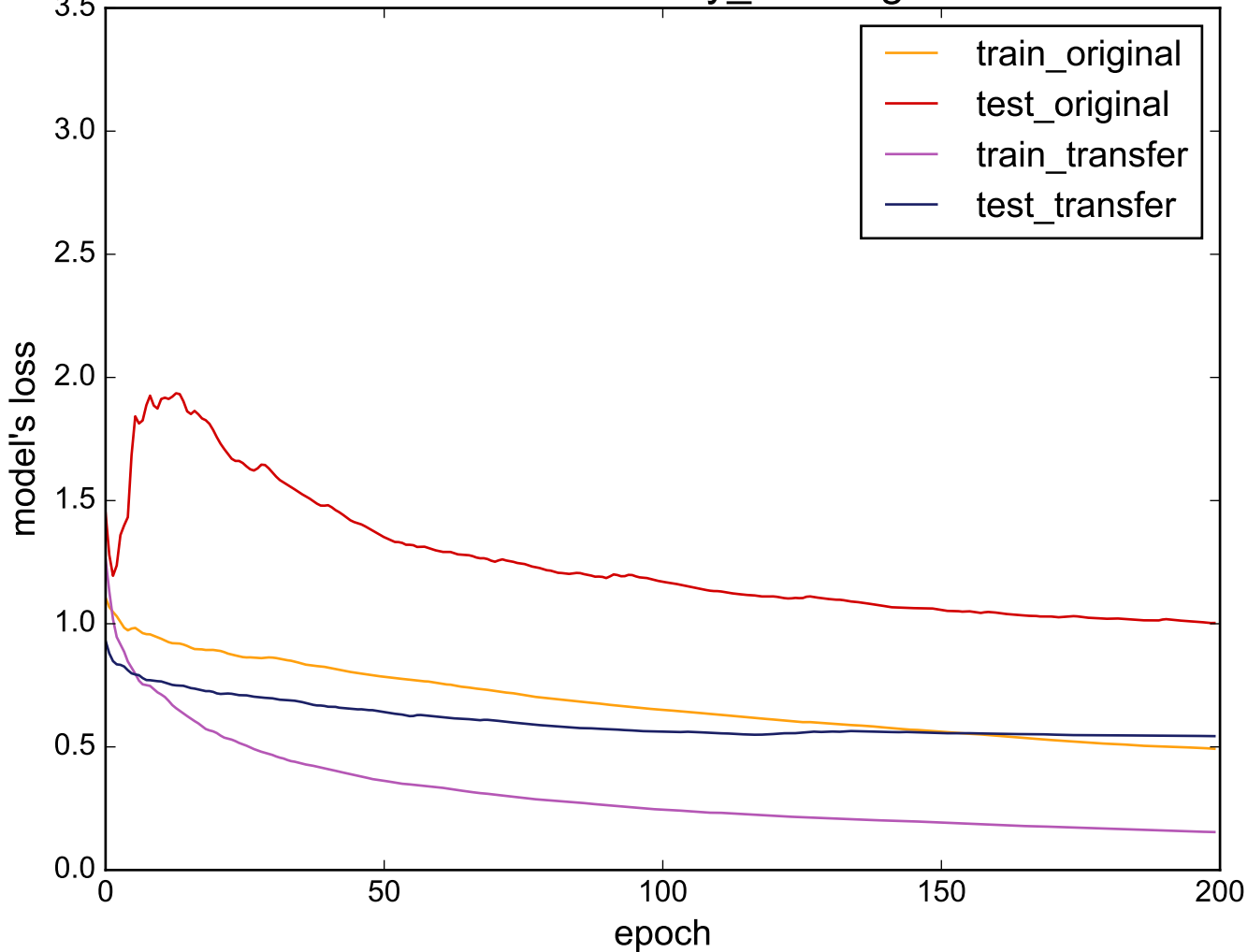
Source: uWaveGestureLibrary_Z - Target: ArrowHead
