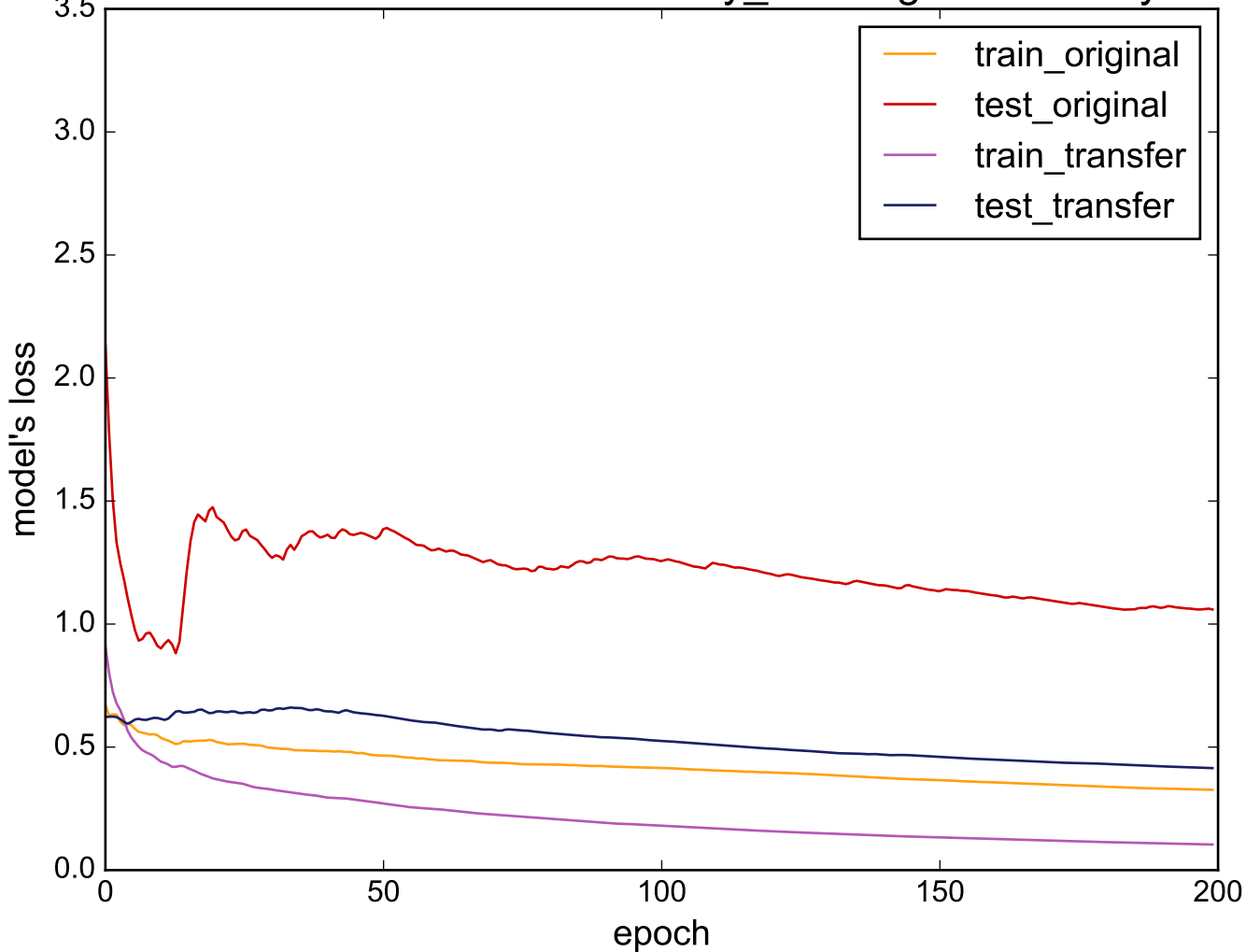
Source: uWaveGestureLibrary_Z - Target: BeetleFly
