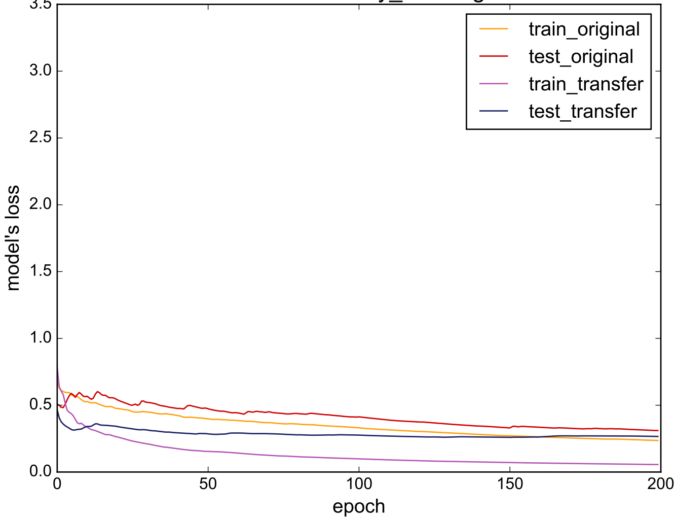
Source: uWaveGestureLibrary_Z - Target: BirdChicken
