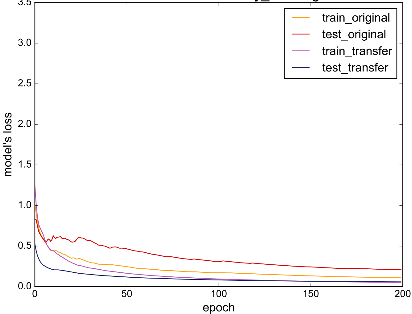
Source: uWaveGestureLibrary_Z - Target: CBF
