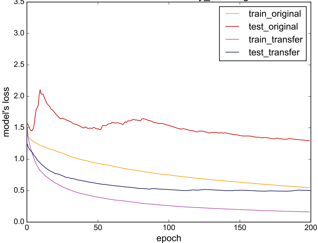
Source: uWaveGestureLibrary_Z - Target: Car
