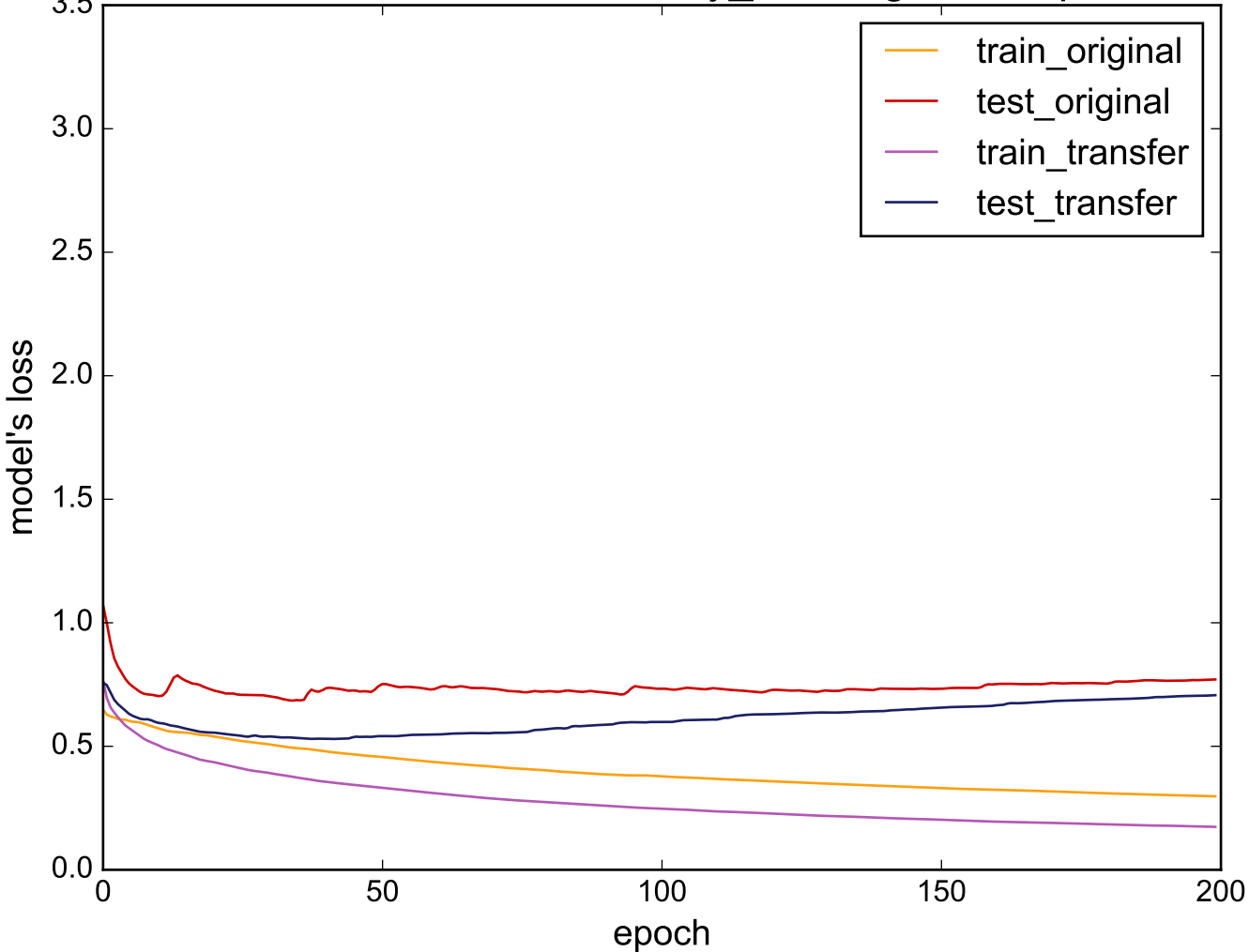
Source: uWaveGestureLibrary_Z - Target: Computers
