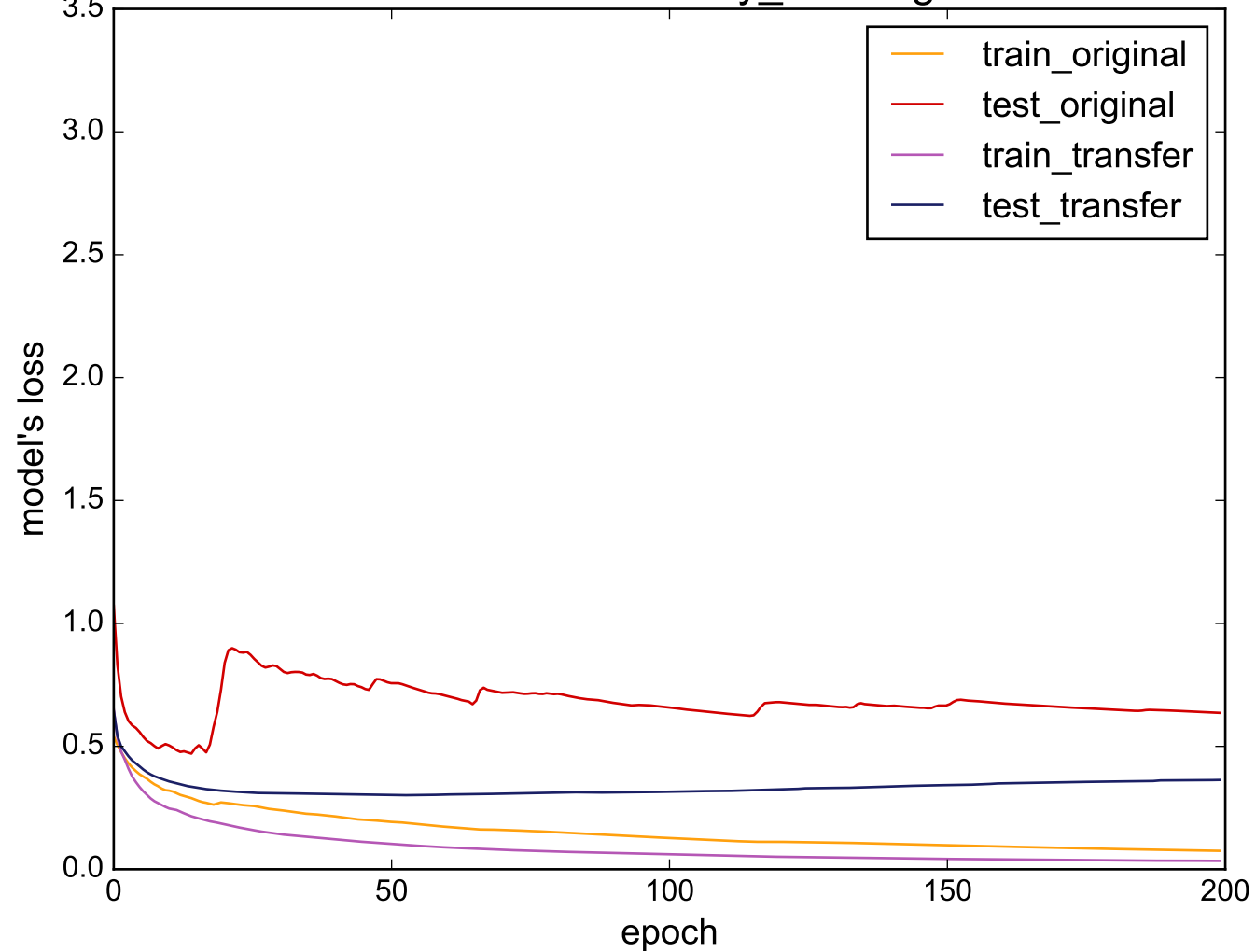
Source: uWaveGestureLibrary_Z - Target: ECG200
