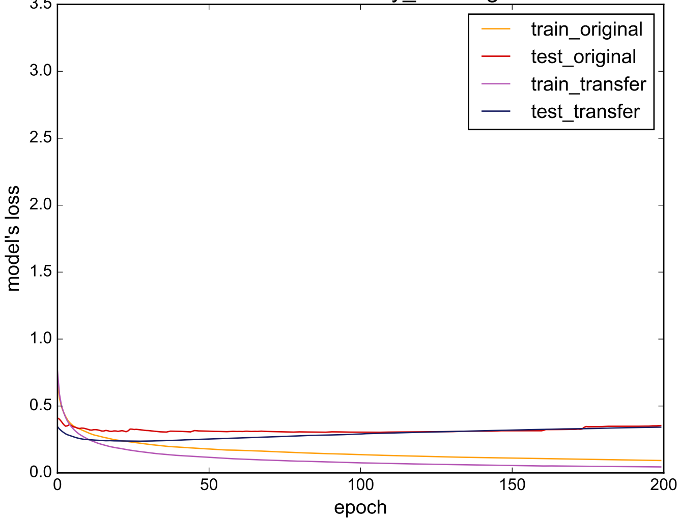
Source: uWaveGestureLibrary_Z - Target: ECG5000
