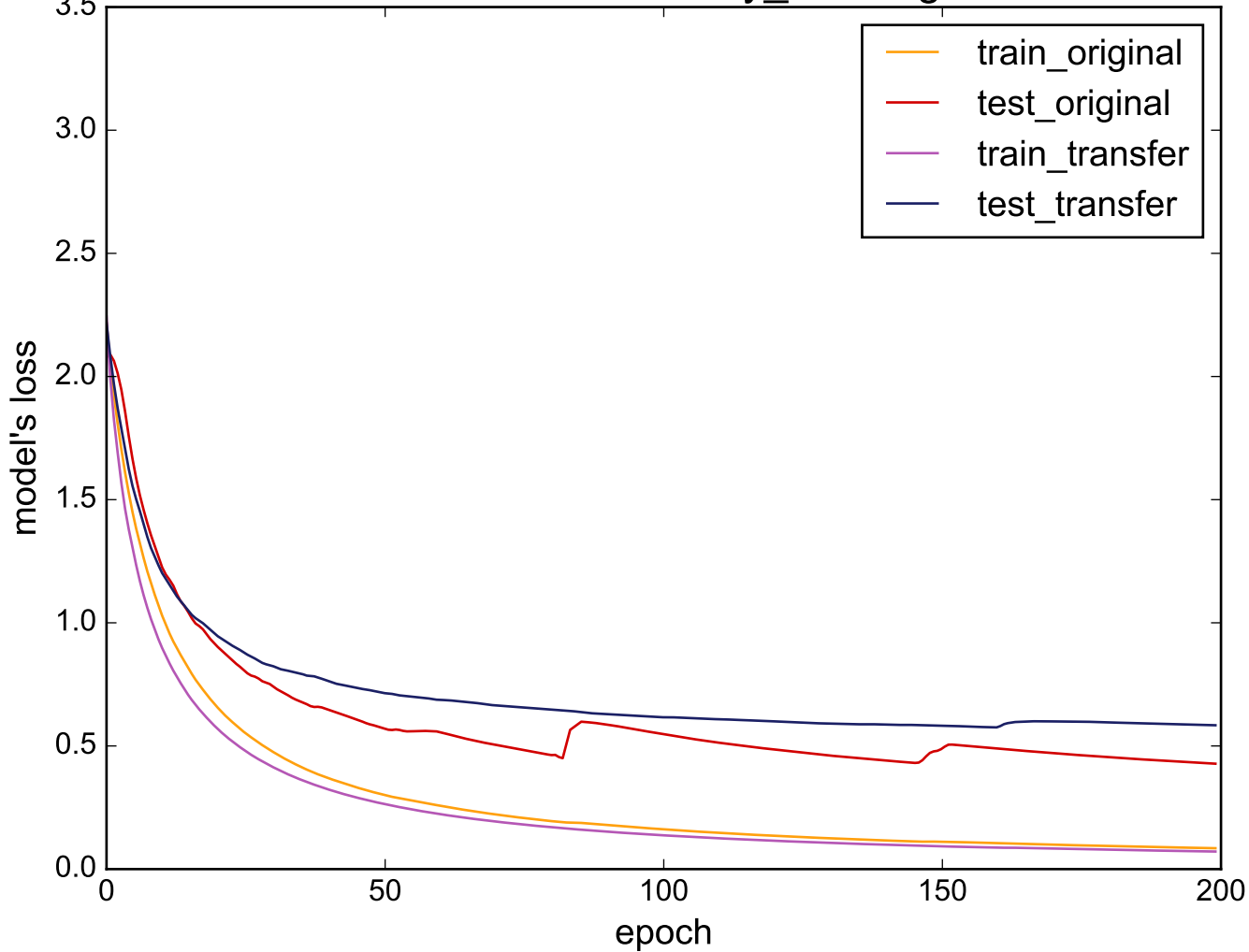
Source: uWaveGestureLibrary_Z - Target: FaceAll
