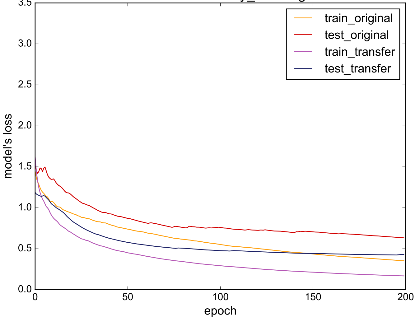
Source: uWaveGestureLibrary_Z - Target: FaceFour
