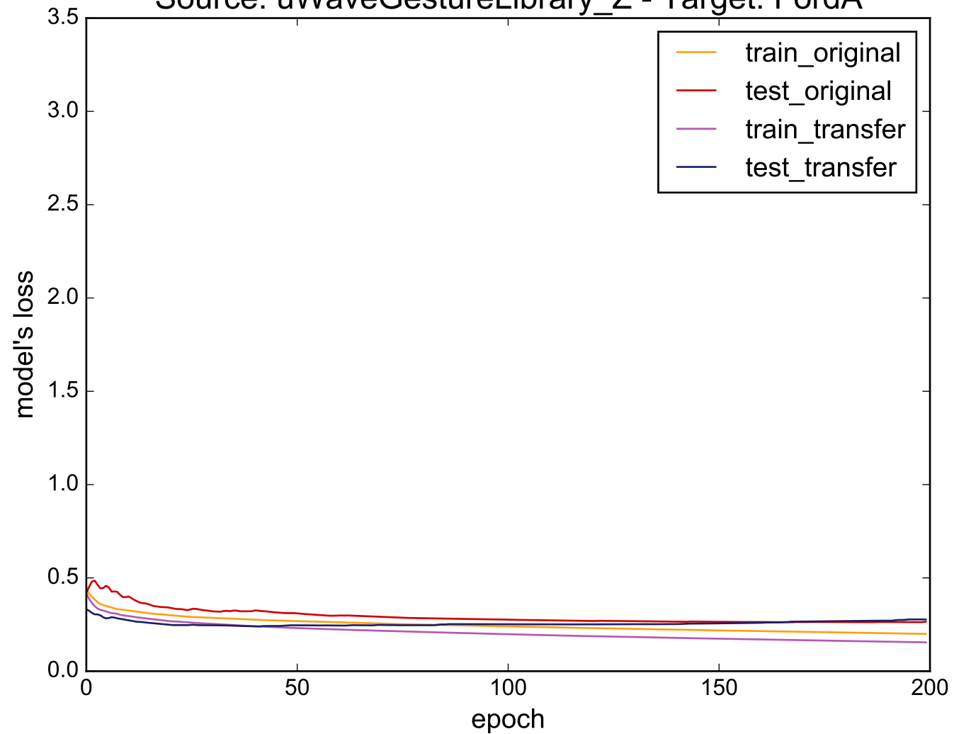
Source: uWaveGestureLibrary_Z - Target: FordA
