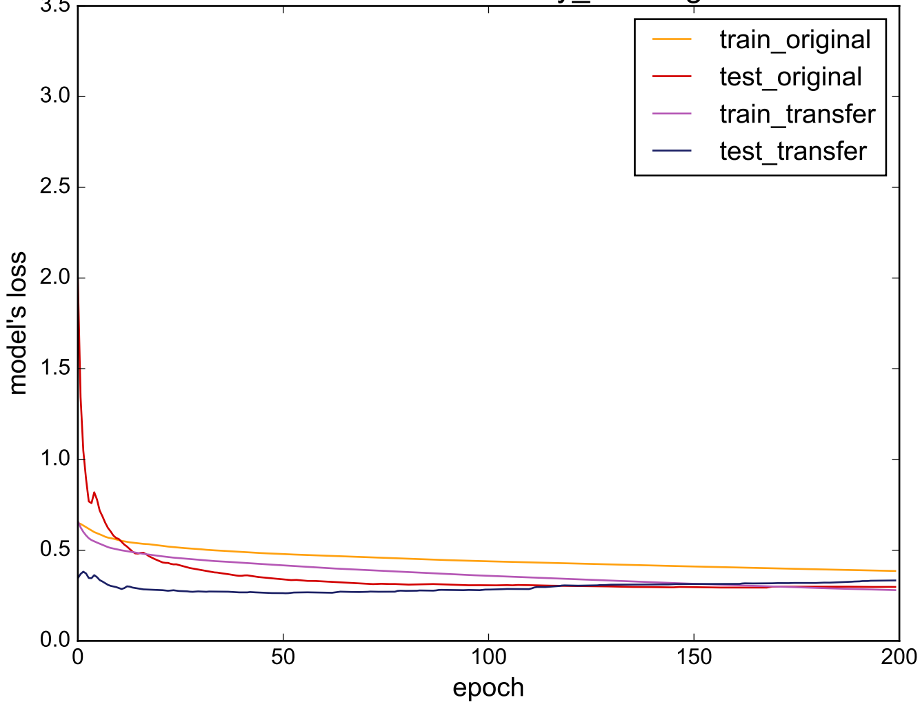
Source: uWaveGestureLibrary_Z - Target: FordB
