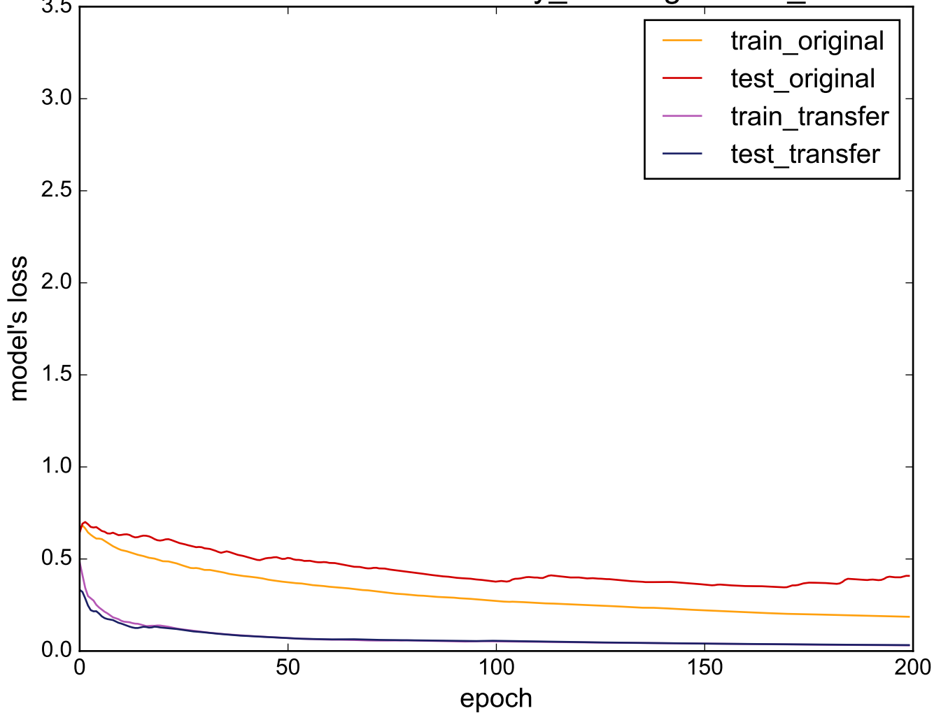
Source: uWaveGestureLibrary_Z - Target: Gun_Point
