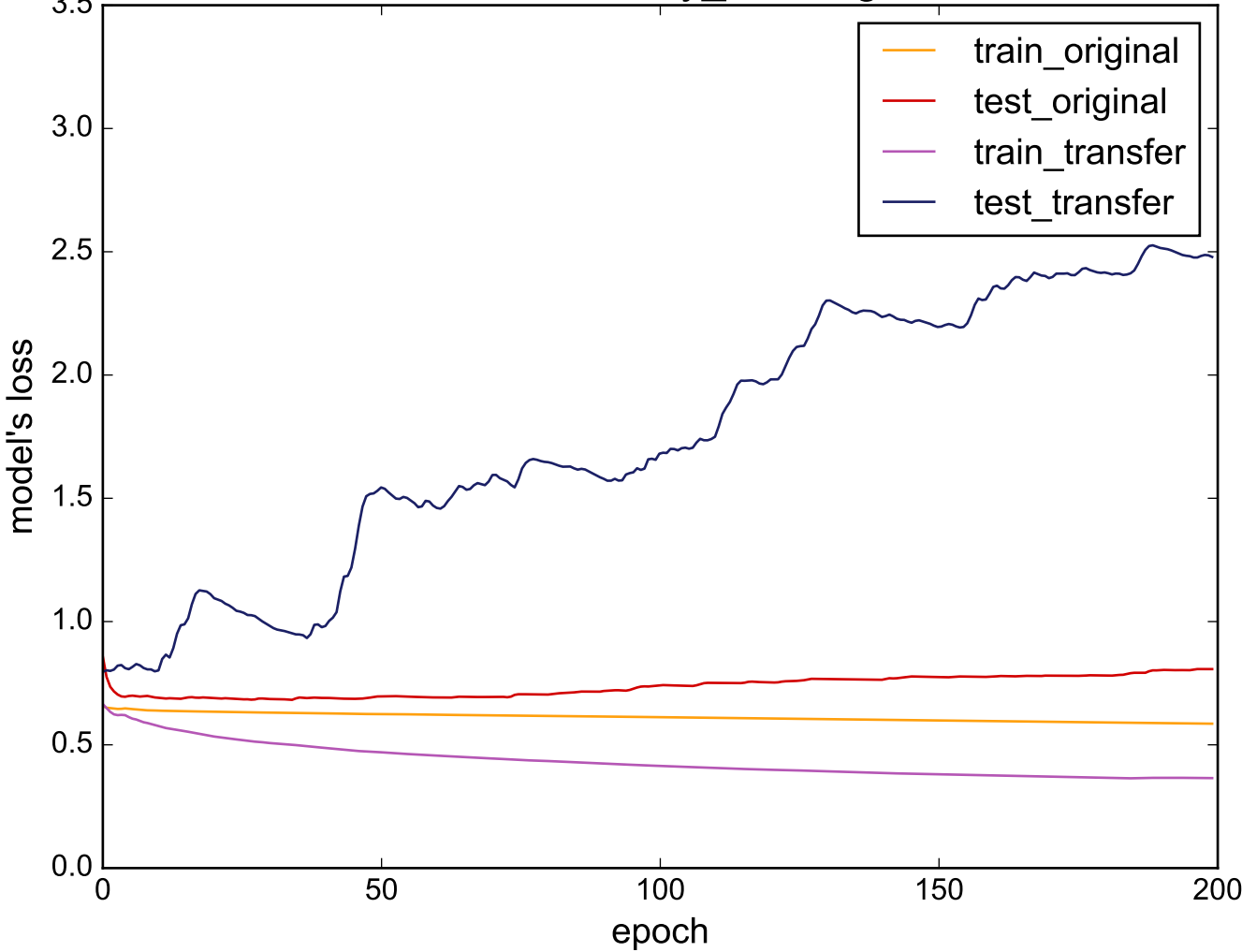
Source: uWaveGestureLibrary_Z - Target: HandOutlines
