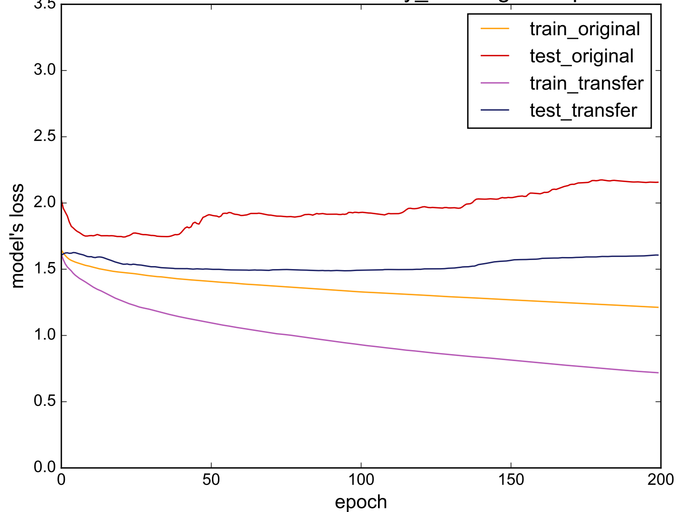
Source: uWaveGestureLibrary_Z - Target: Haptics
