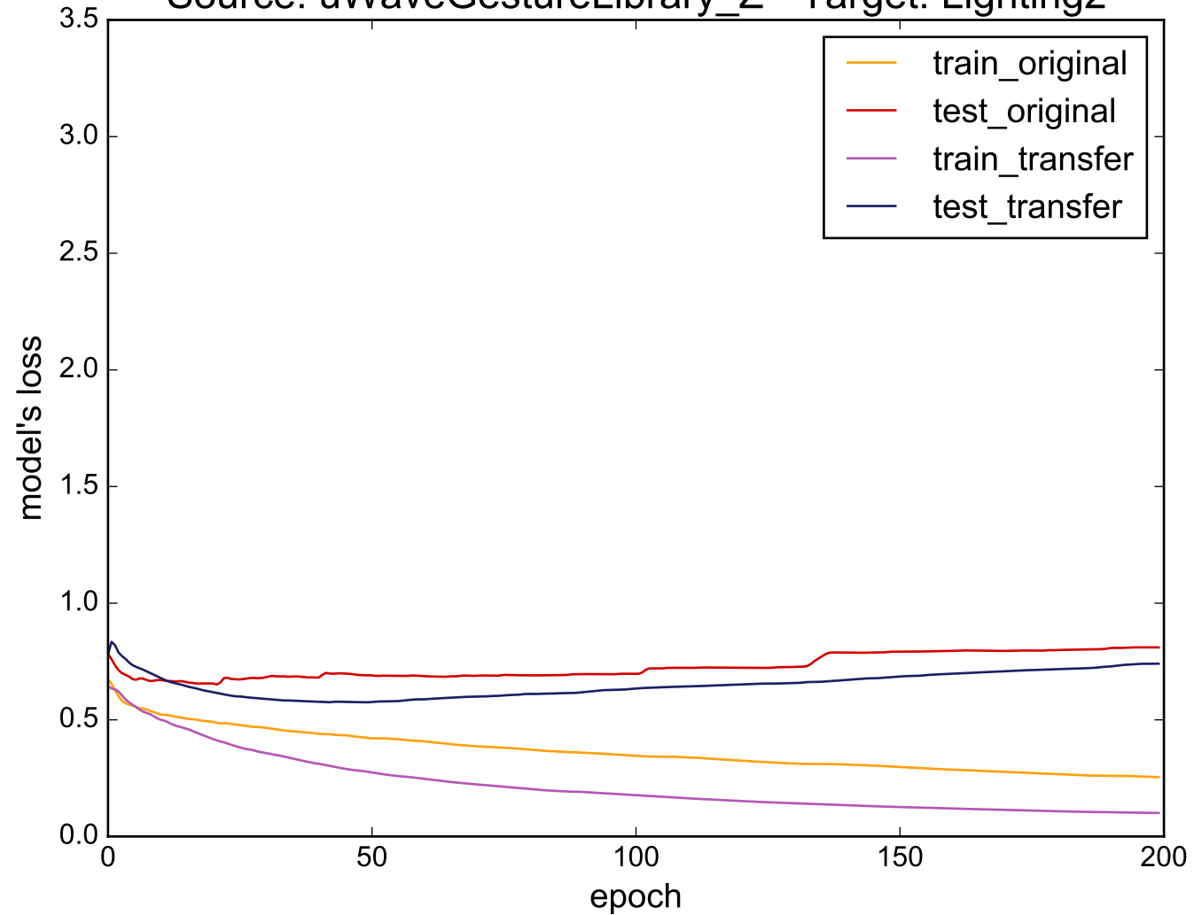
Source: uWaveGestureLibrary_Z - Target: Lighting2
