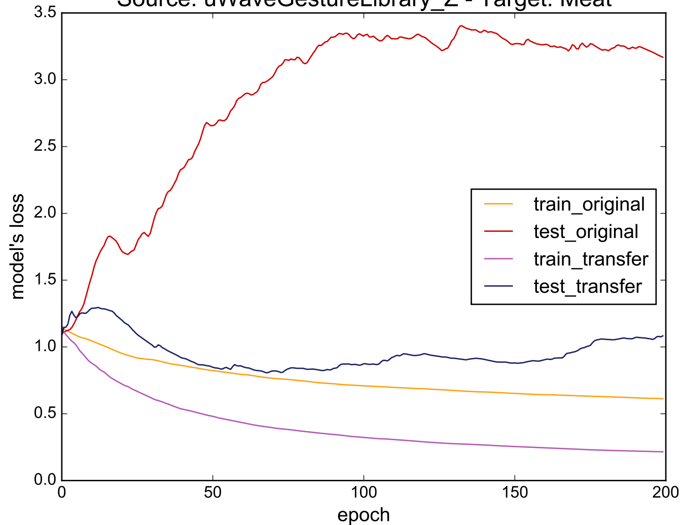
Source: uWaveGestureLibrary_Z - Target: Meat
