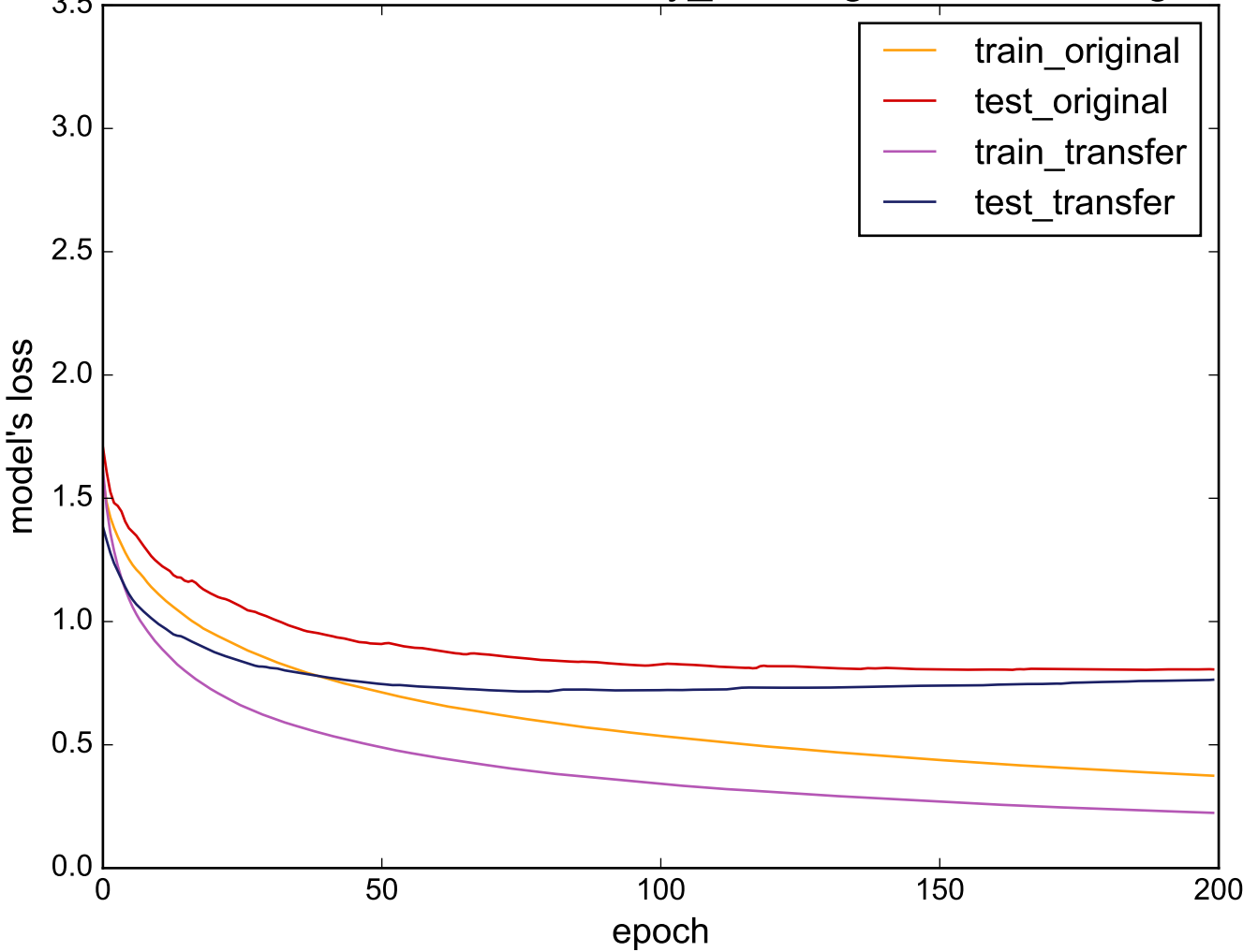
Source: uWaveGestureLibrary_Z - Target: MedicalImages
