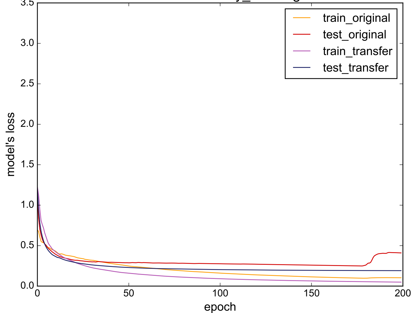
Source: uWaveGestureLibrary_Z - Target: MoteStrain
