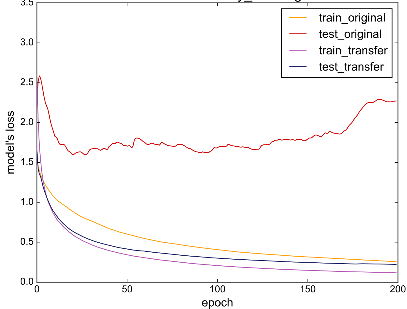
Source: uWaveGestureLibrary_Z - Target: OSULeaf
