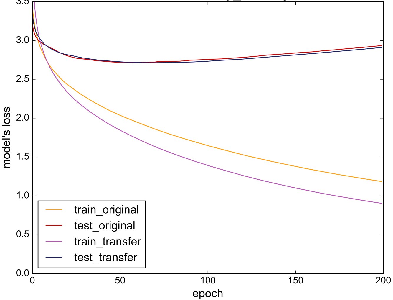
Source: uWaveGestureLibrary_Z - Target: Phoneme
