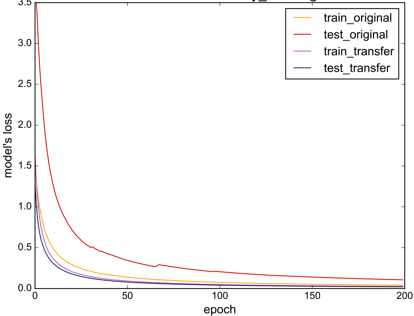
Source: uWaveGestureLibrary_Z - Target: Plane
