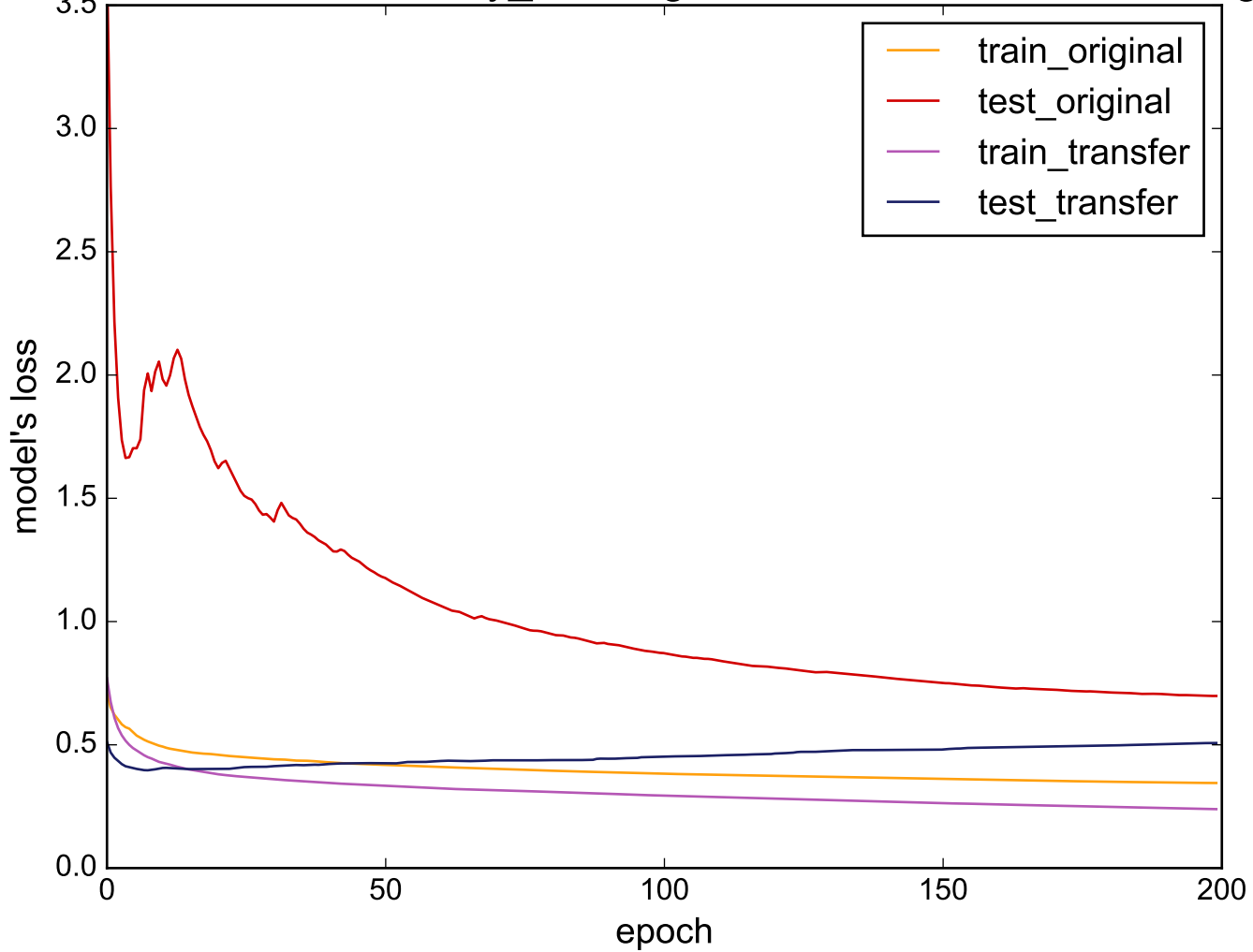
Source: uWaveGestureLibrary_Z - Target: ProximalPhalanxOutlineAgeGroup
