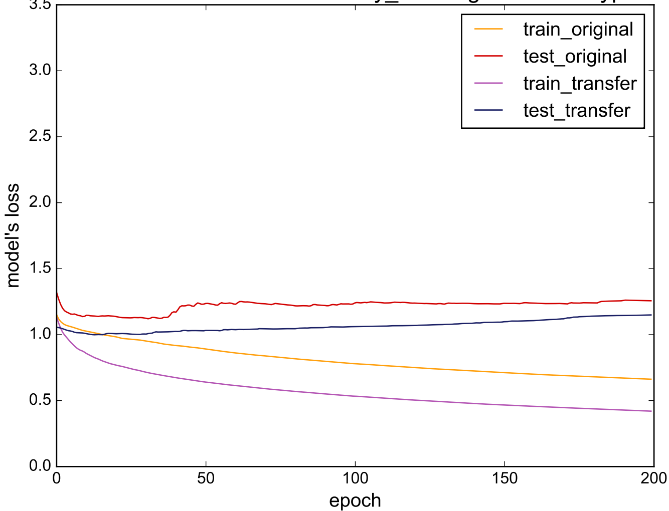
Source: uWaveGestureLibrary_Z - Target: ScreenType
